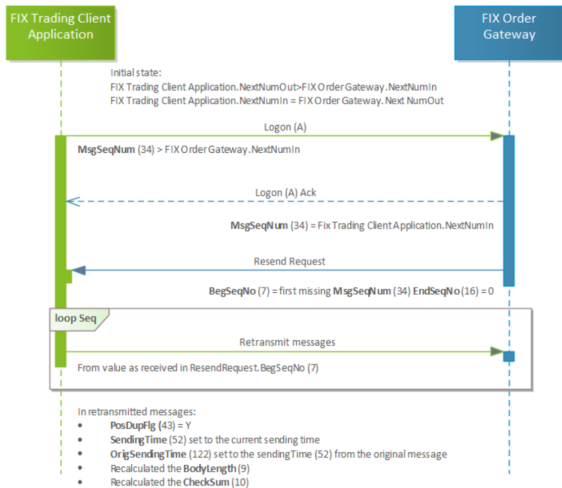
Figure 6 – Logon with gap fill procedure
